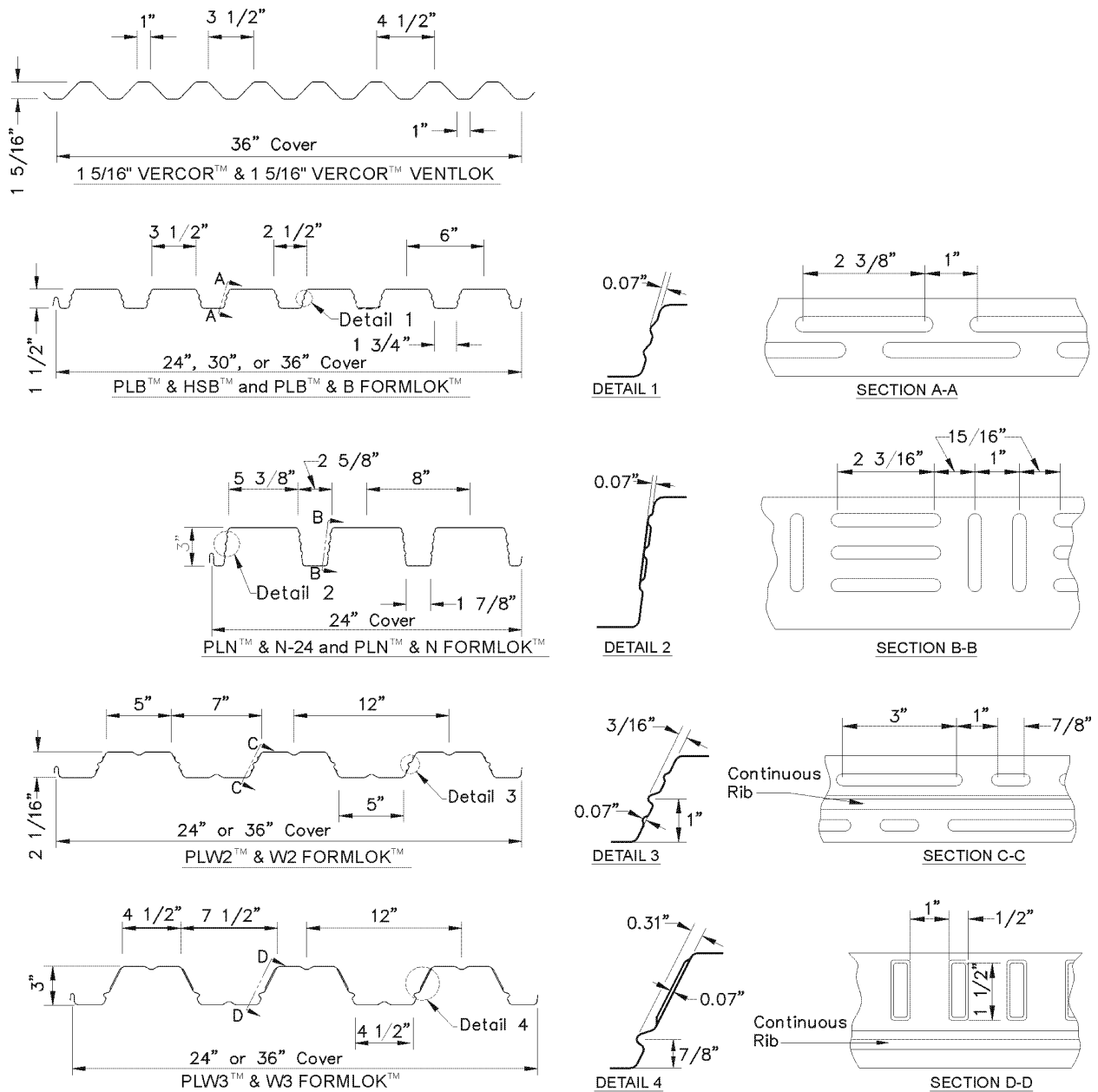
FIGURE 1-DECK PROFILES
