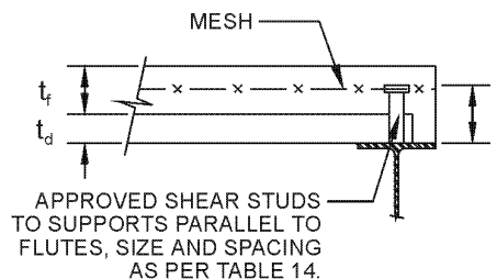
SHEAR STUDS AT SUPPORTS PERPENDICULAR TO FLUTES
